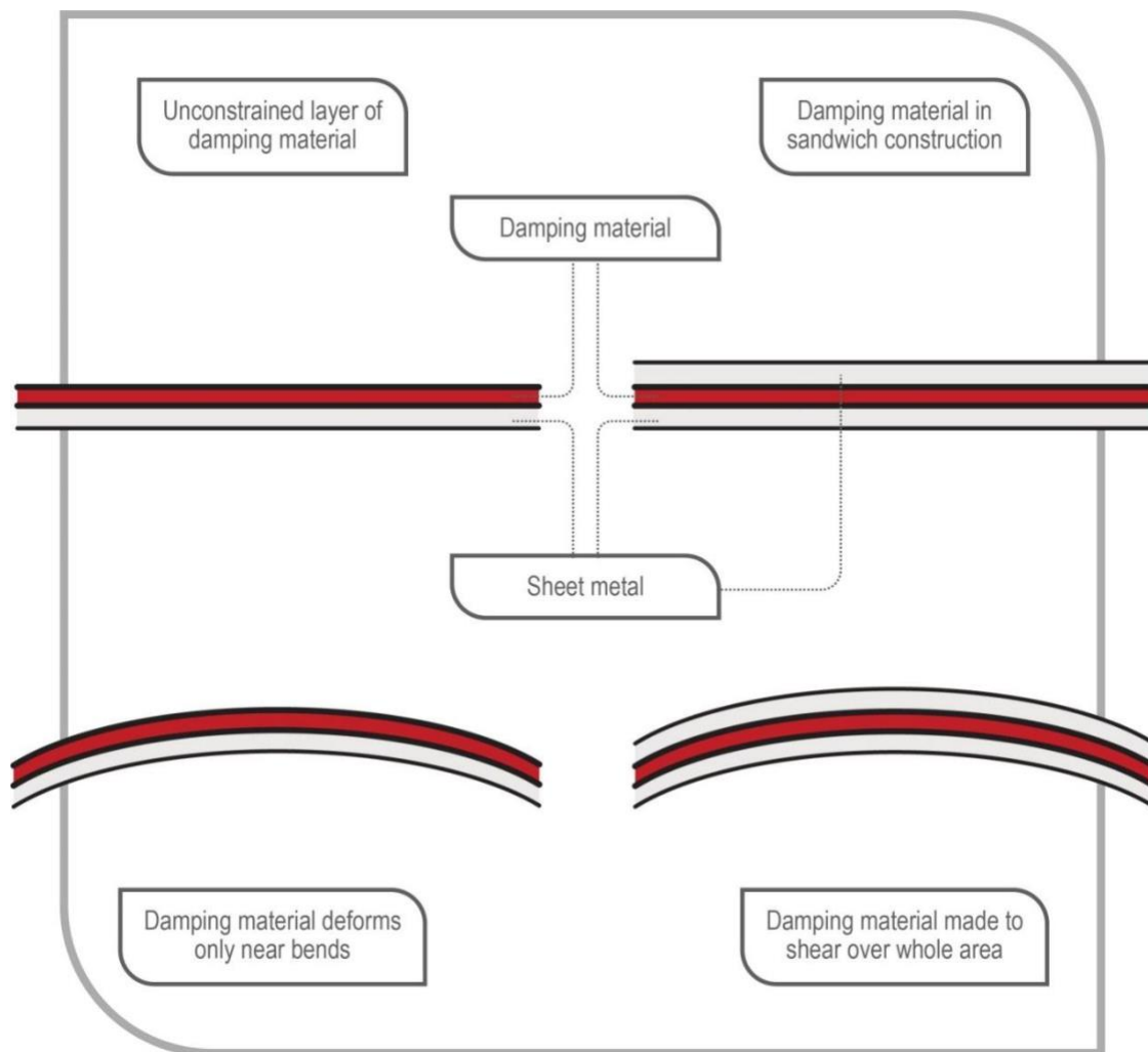
Figure 4 Damping
