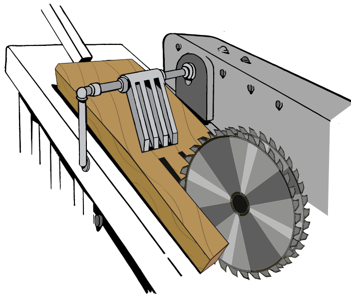
Figure 10: Anti-kickback device.
