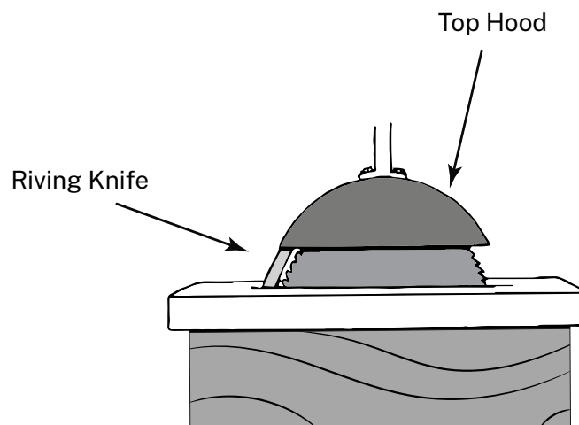
Figure 13: The riving knife should be as close to the blade as possible.
