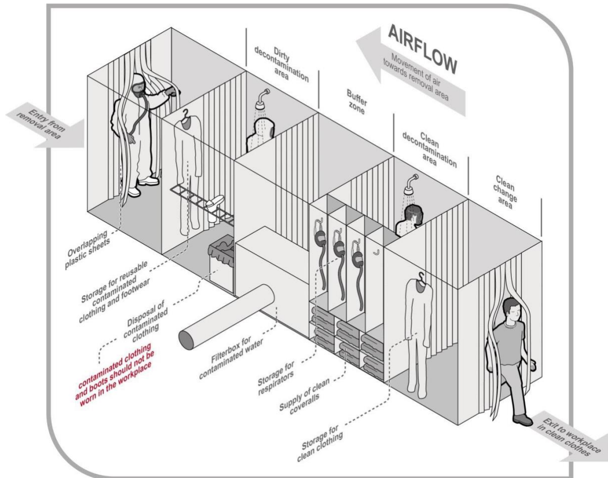
Figure 4 Decontamination unit
