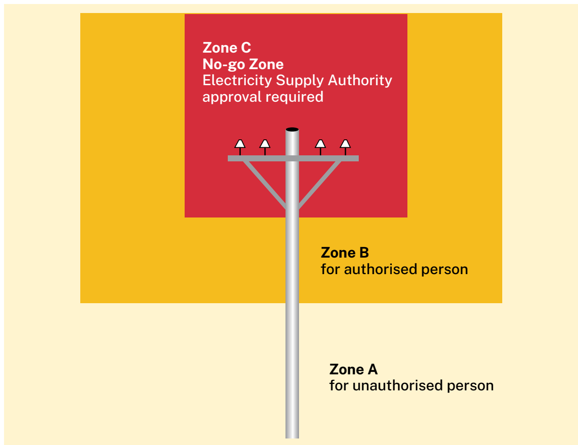
Figure 10 Work zones for EWPs near overhead electric lines
