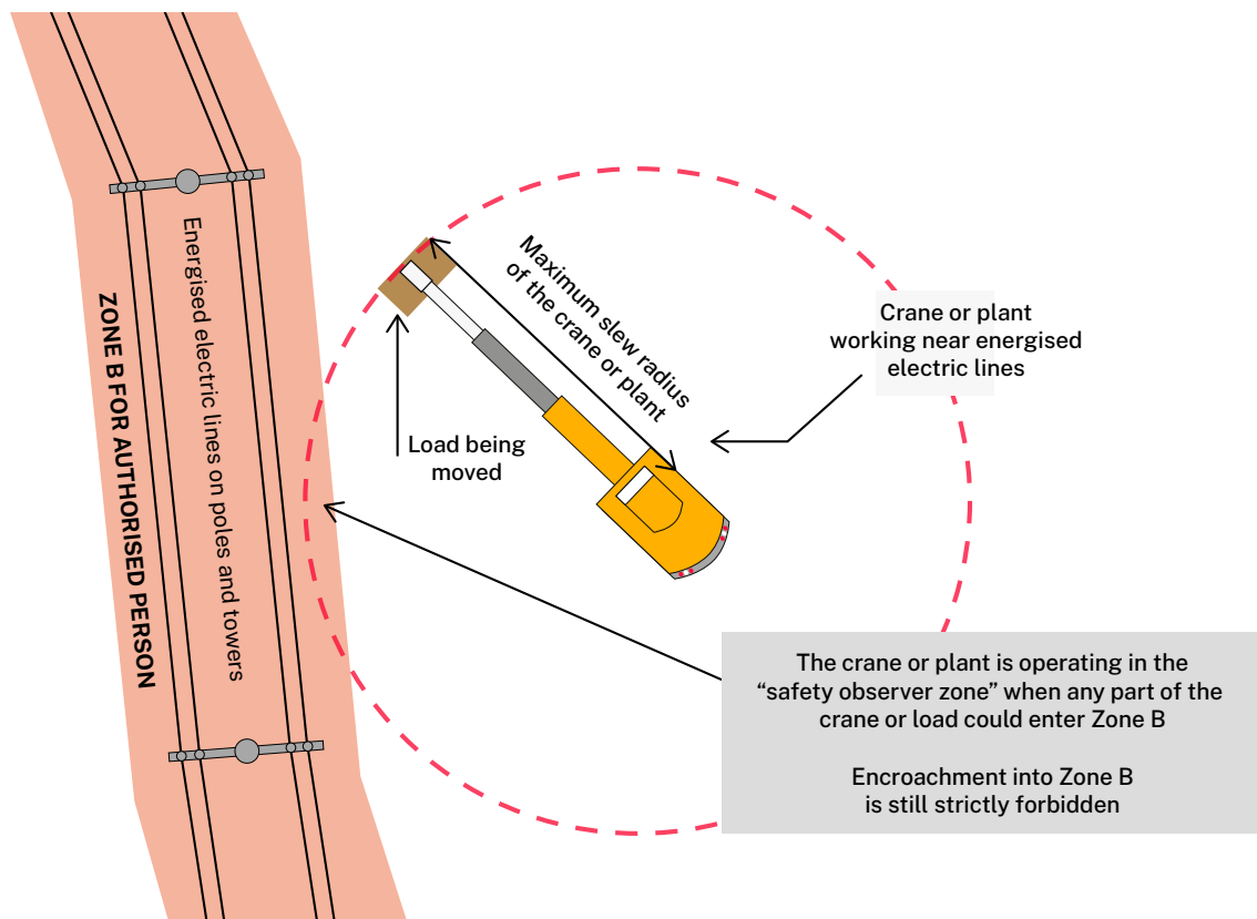
Figure 11 Operations near overhead electric lines
