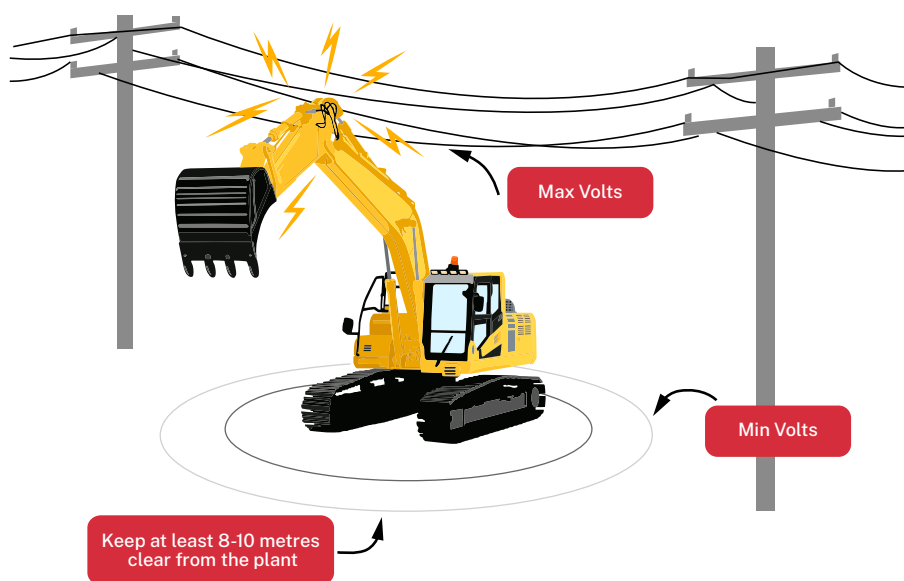
Figure 21: Affected area surrounding mobile plant when in contact with live overhead electric line
