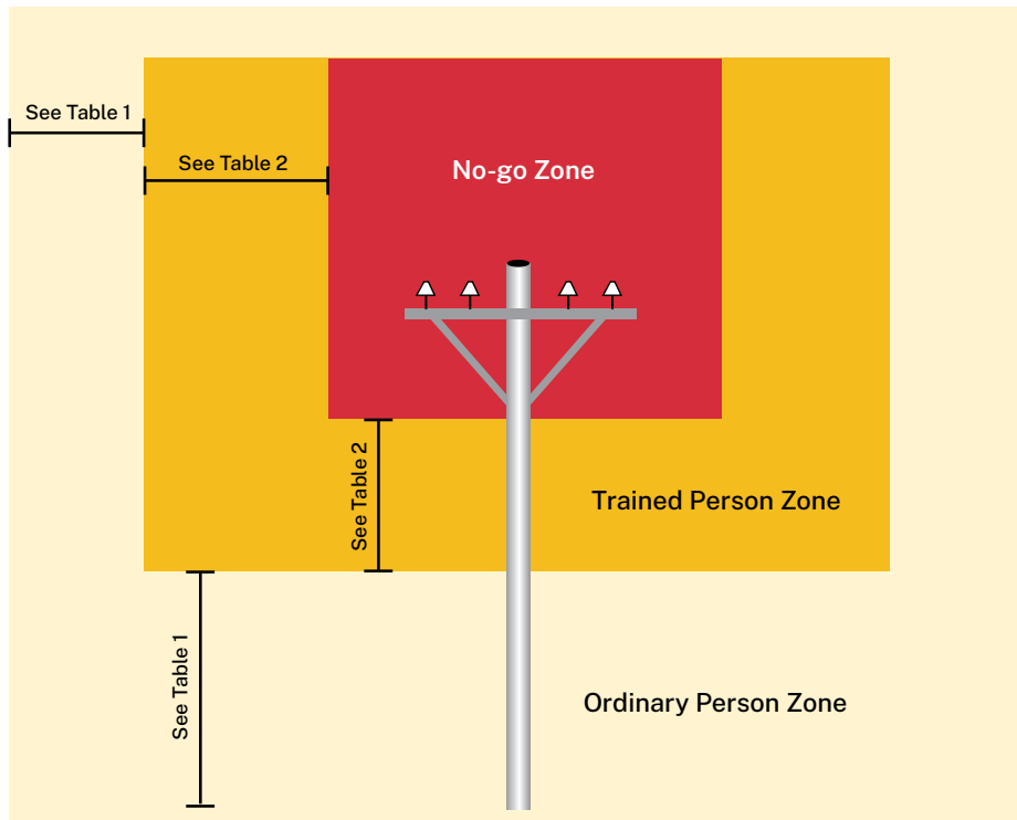
Figure 5: Approach distances and work zones near overhead electric lines
