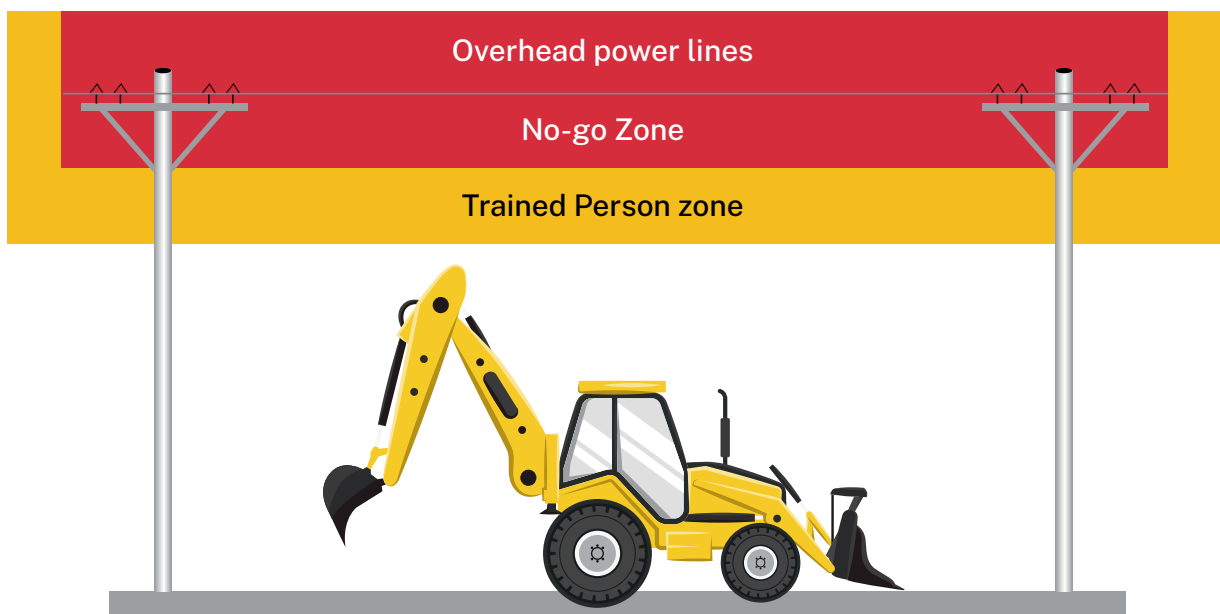
Figure 7: Cranes and mobile plant working near overhead electric lines
