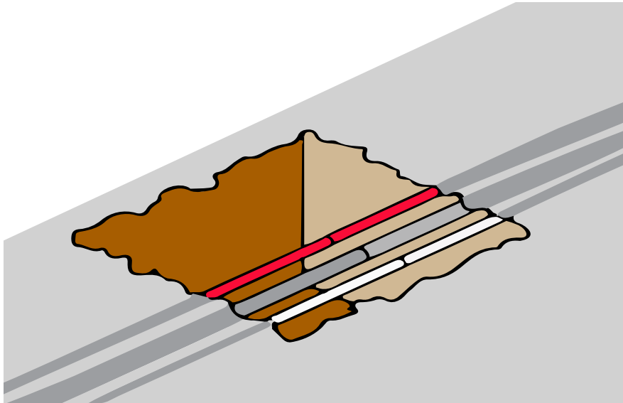
Figure 17 - Underground essential services exposed by potholing
