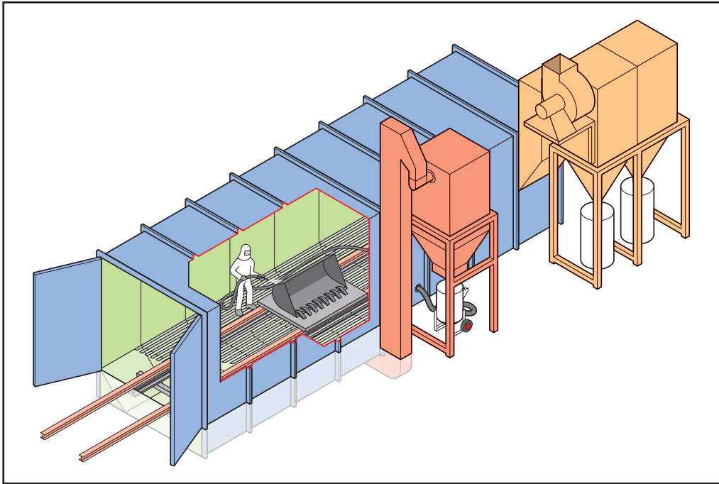
Blasting chamber
